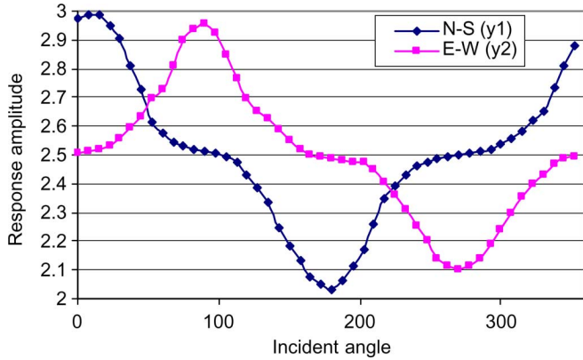
Fig. 2. Excessive element separation distances lead to an approximate \sin^3 and \cos^3 response as a reduction of sensitivity is introduced at angles perpendicular to the particular axis (actual recorded response).
