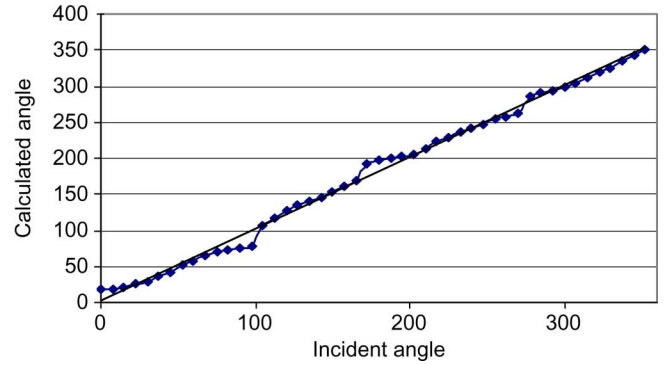
Fig. 3. Calculated solution for the \sin^3/\cos^3 characteristic response of Fig. 2.
