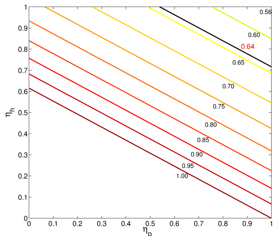
FIG. 4: The pale contours indicate the value of \eta required to demonstrate steering with inefficient homodyne and photodetection measurements. For lower measurement efficiencies there are no contours, as it would require unphysical values of \eta (i.e. \eta > 1 ) to satisfy the steerability criterion. The black contour ( \eta = 0.64 ) marks the preparation efficiency limit achieved experimentally in [10].
