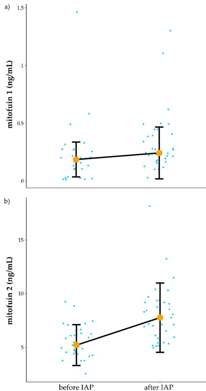
Figure 4. Influence of IAP on Mitofusins. (a) influence of IAP on mitofusin1 level. (b) influence of IAP on mitofusin2 level. IAP—Individualised Activity Program, Orange dots connected by black line indicate median value, vertical black lines denote interquartile range. Blue dots before and after denote the results of individual patients.
