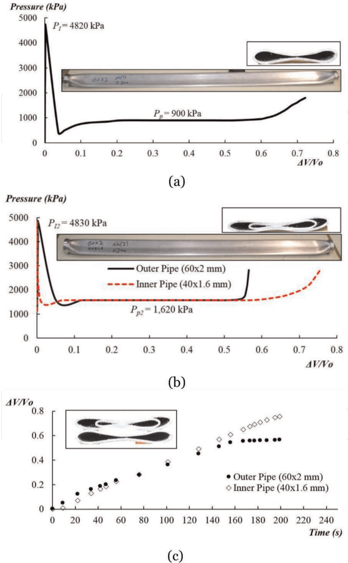
Figure 8. Buckle propagation response inside the hyperbaric chamber: (a) pressure versus normalized change of volume of the 60 x 2 mm carrier pipe, (b) pressure versus normalized change of volume of PIP-2 and (c) normalized volume versus time of PIP-2.
