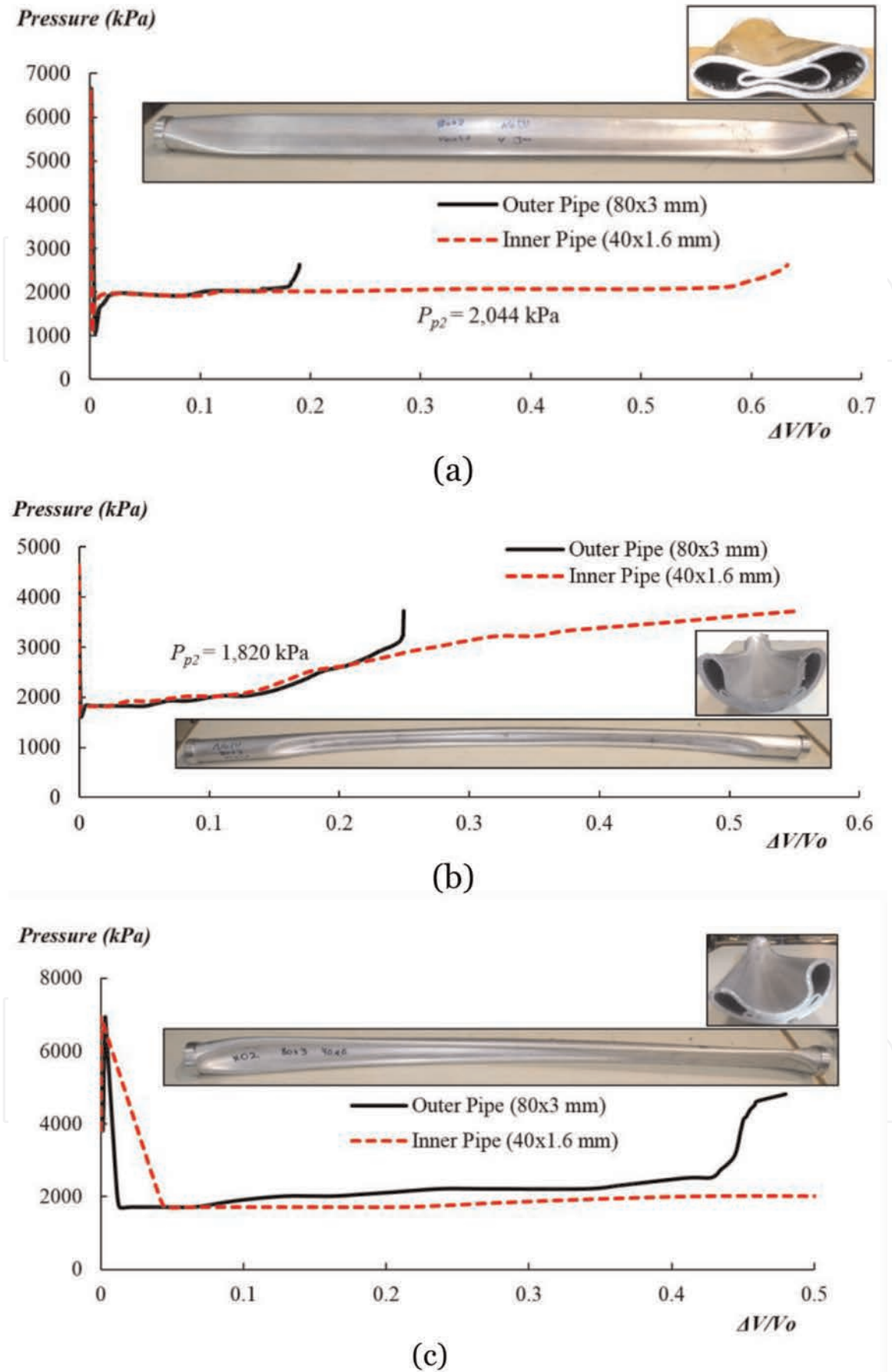
Figure 10. Buckle propagation response inside the hyperbaric chamber: (a) buckle propagation response of the PIP-3 ( 80 \times 3 \text{ mm}-40 \times 1.6 \text{ mm} ) with dog-bone buckle shape, (b) buckle propagation response of PIP-3 with confined buckle shape and (c) buckle propagation response of PIP-3 showing interaction between dog-bone and confined buckle shape.
