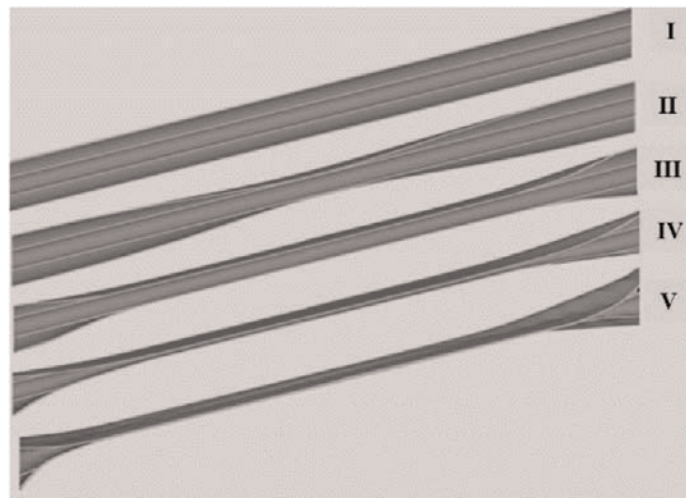
Figure 13. Finite element results showing pressure against normalized ovality and corresponding deformed shapes of PIP system exhibiting buckle propagation mode B.
