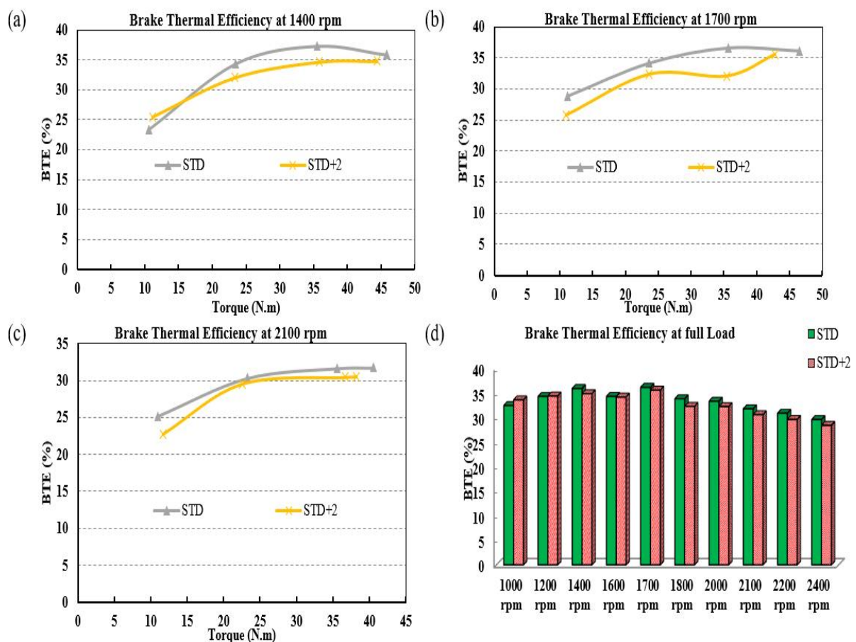
Figure 2. Brake Thermal Efficiency of the engine running with WCO for standard (STD) and retard injection timings (STD+2) at (a) 1400 rpm, (b) 1700 rpm, (c) 2100 rpm and (d) full load.
