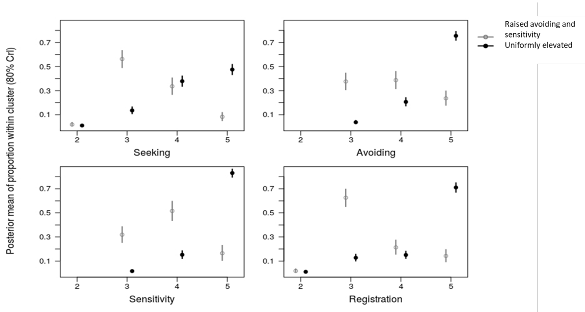
Figure 2. Posterior summary of proportion of sample contained in each cluster. Posterior mean identified by open/closed circles and indicated spread denotes 80% credible interval.
