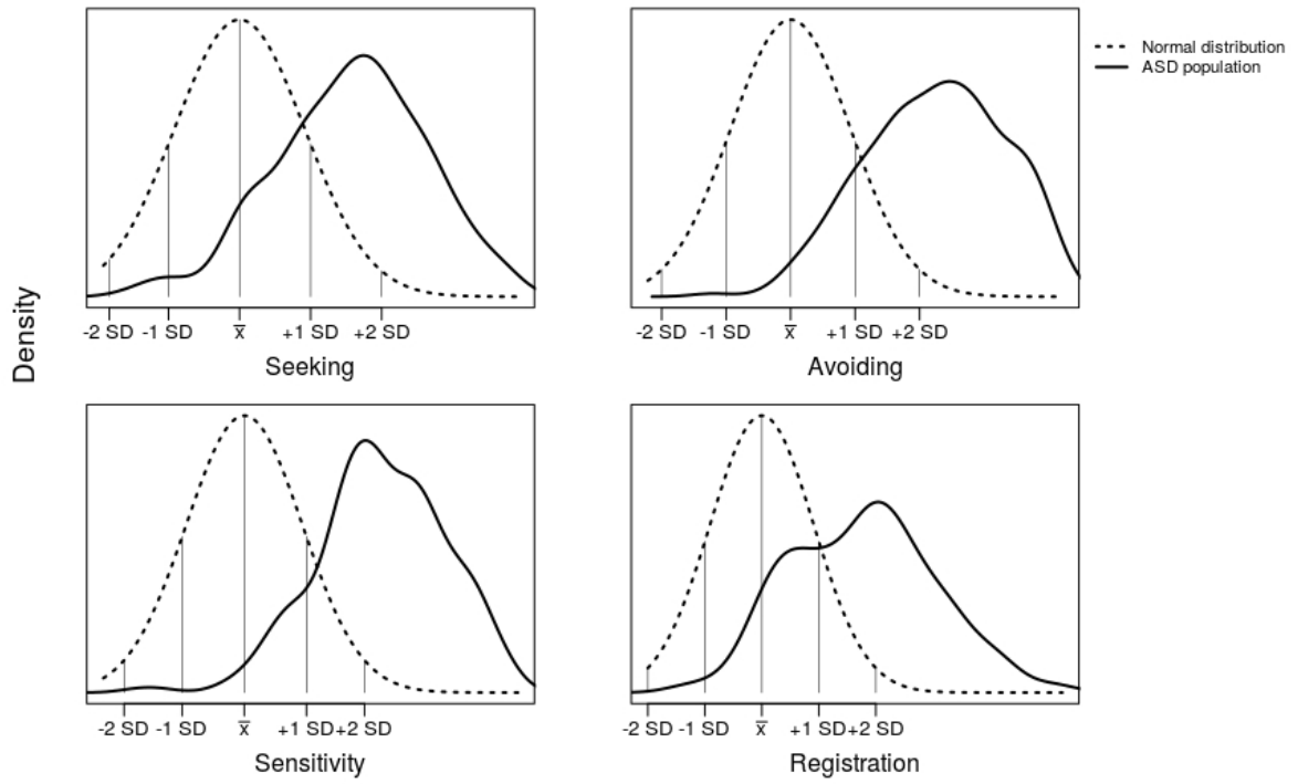
Figure 1. Distribution of participant quadrant scores compared with the Normal Curve and Sensory Profile 2 Classification System.
