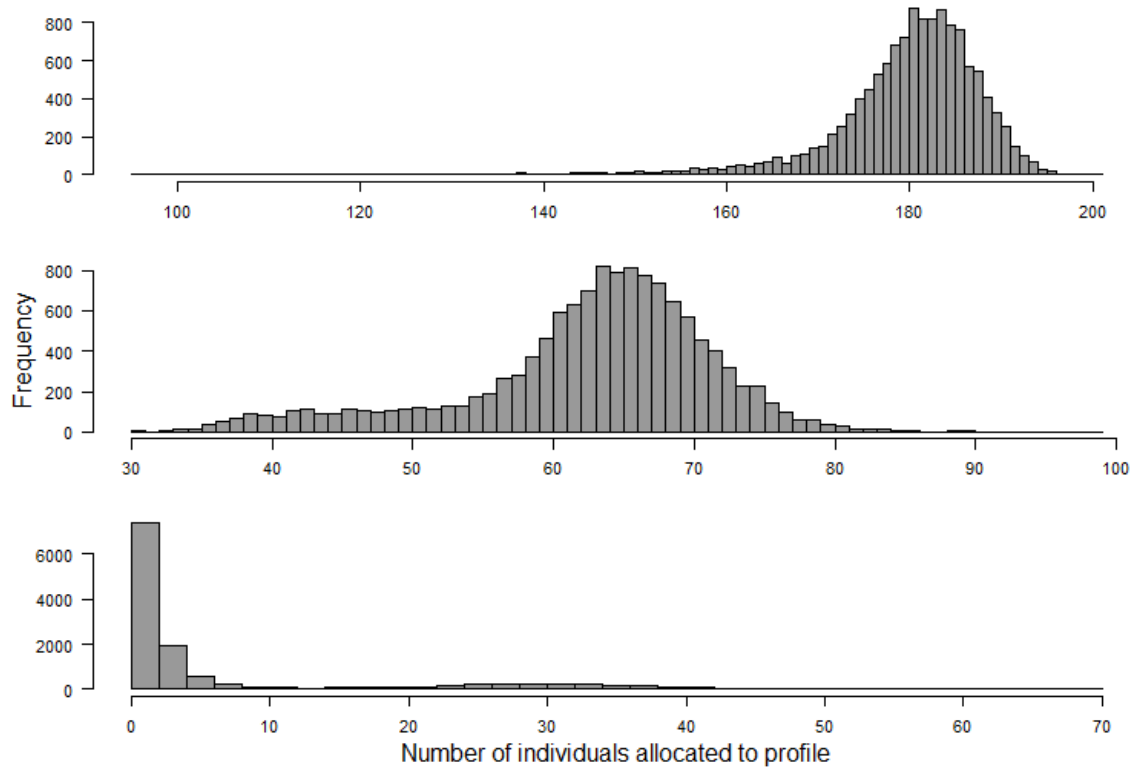
Figure 3. Histograms of number of individuals assigned to each profile over 12,839 iterations of the sampler containing three components. Top Panel: Uniformly elevated, Middle Panel: Raised avoiding and sensitivity, Bottom Panel: Extra 1 and 2.
