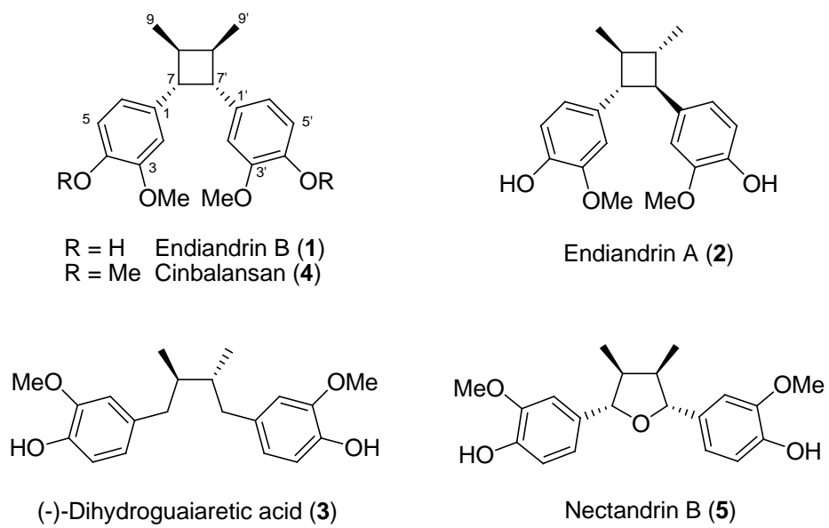
Figure 1. Chemical structures for compounds 1-5.
