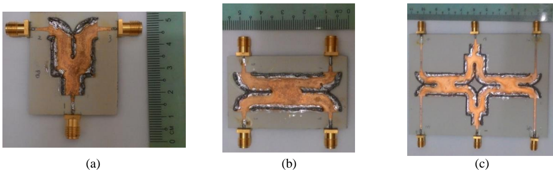
Figure 4. Photograph of the fabricated (a) SIW power divider, (b) SIW hybrid coupler, (c) SIW six-port
