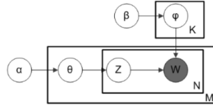
Fig. 1: The structure of Latent Dirichlet Allocation
