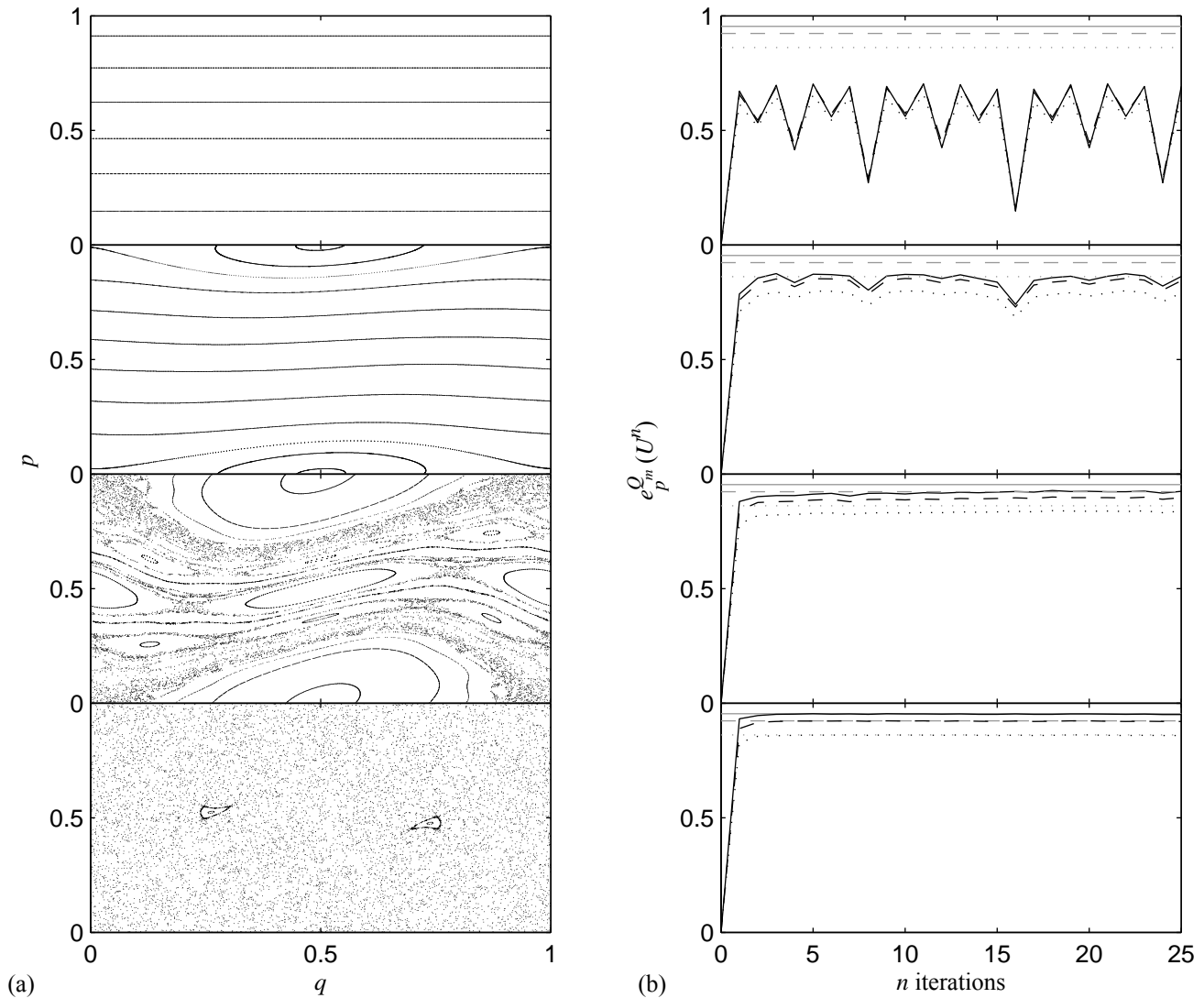
FIG. 1: (a) Phase-space portraits of the classical kicked rotor for k = 0, 0.2, 1 and 6 (from top to bottom), and (b) the corresponding entangling power in the quantum case. A Hilbert space of 6 qubits was chosen allowing the investigation of the multipartite entanglement measures Q_m for m = 1 (dotted), 2 (dashed) and 3 (full). The average entanglement for random states is shown in the lighter tones.
