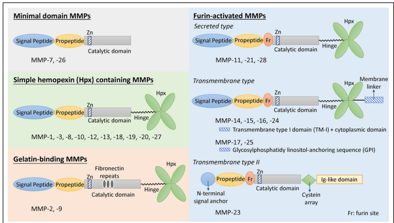
Figure 2. Domain structure of MMPs. Most MMPs share a similar basic structure: a signal peptide, a propeptide, a zinc-containing catalytic domain, hemopexin (Hpx) domain, and a hinge region. MMP-7 and MMP-26 are the smallest MMPs with minimal domain structure, lacking Hpx domain and hinge region. Gelatin-binding MMPs (MMP-2 and MMP-9) contain three fibronectin repeats in their catalytic domain. Furin-activated MMPs (including secreted MMPs, transmembrane MMPs, and one transmembrane type II MMP) contain a furin recognition site. Transmembrane-type MMPs contain a transmembrane domain and a cytoplasmic domain or a glycosylphosphatidylinositol linkage (GPI). The transmembrane-type II MMP (i.e., MMP-23) has a signal anchor at N-terminal, and a cysteine array and an immunoglobulin (Ig)-like domain at C-terminal.
