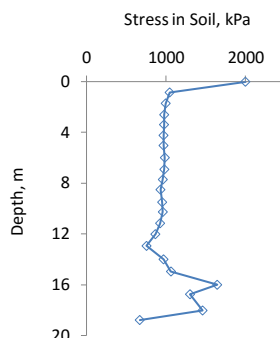
Fig. 9. Stress in soil
