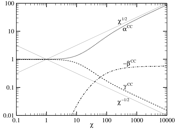
FIG. 4. The parameters for the closest-to-coherent physically-realizable (CC PR) ensemble as a function of \chi similar to Fig. 2 but here with \nu = 100 . The excess phase diffusion allows the realization of states very close to coherent states until \chi \sim \nu^{1/2} .
