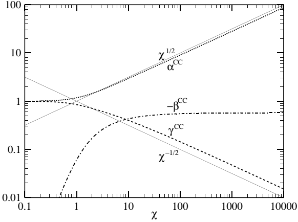
FIG. 2. The parameters for the physically-realizable ensemble that is closest to a coherent ensemble (CC) as a function of \chi with \nu = 0 . The ensembles arise from general continuous Markovian unravelings. These parameters are the phase quadrature variance \alpha^{\text{CC}} (dotted line), the amplitude-quadrature variance \gamma^{\text{CC}} (dashed line) and the covariance \beta^{\text{CC}} (dash-dot line) for the members of this ensemble. Also shown for comparison are thin solid curves representing \chi^{1/2} and \chi^{-1/2} .
