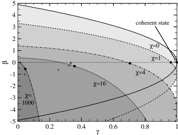
FIG. 3. Representation of physically-realizable ensembles similar to Fig. 1 but for \nu = 10 .
