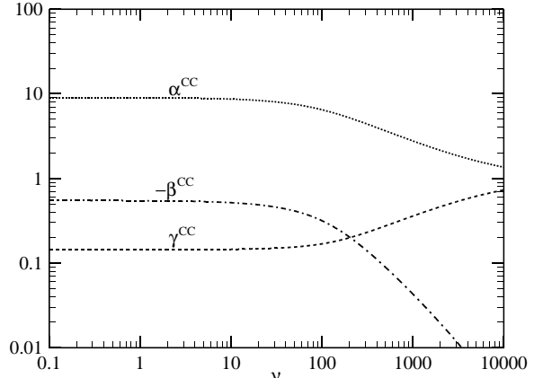
FIG. 5. The parameters of the closest-to-coherent physically-realizable (CC PR) ensemble similar to Fig. 2 but here as a function of \nu and with \chi = 100 .
