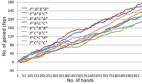
Fig. 2. Performance of PATy over Conservative and Bluffing Players under 8 Configurations
