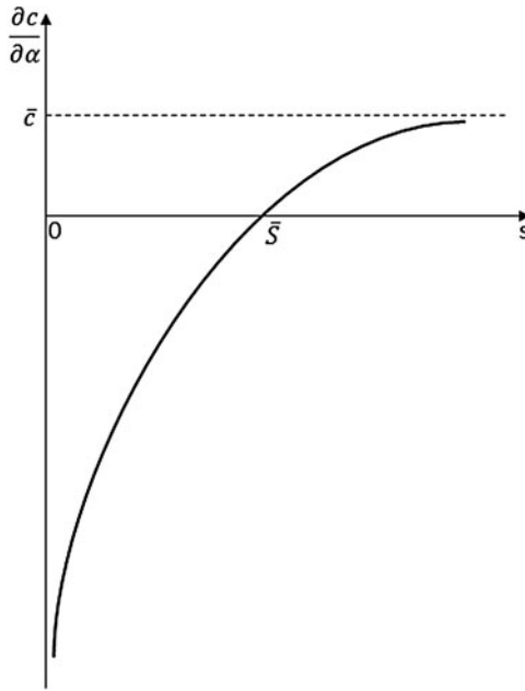
Figure 2. The Relationship Between s and \partial c/\partial \alpha
