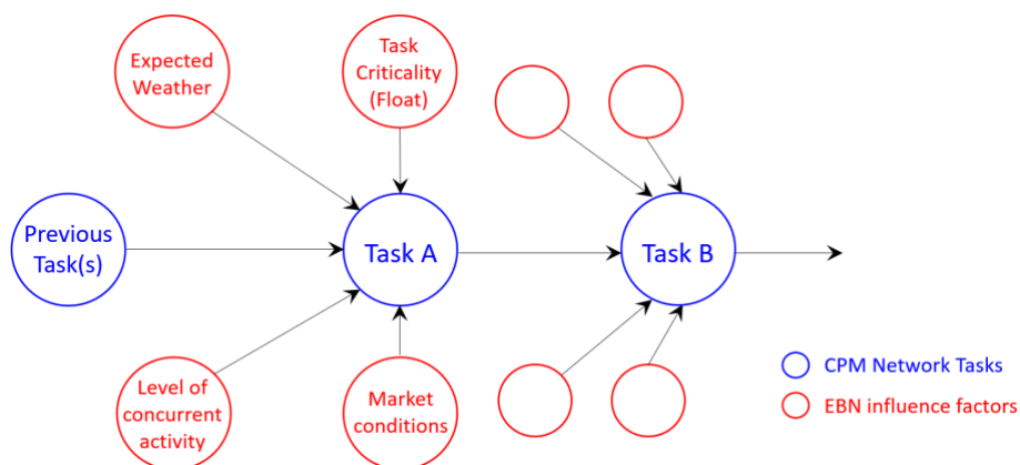
FIG. 5: Bayesian Trigger
