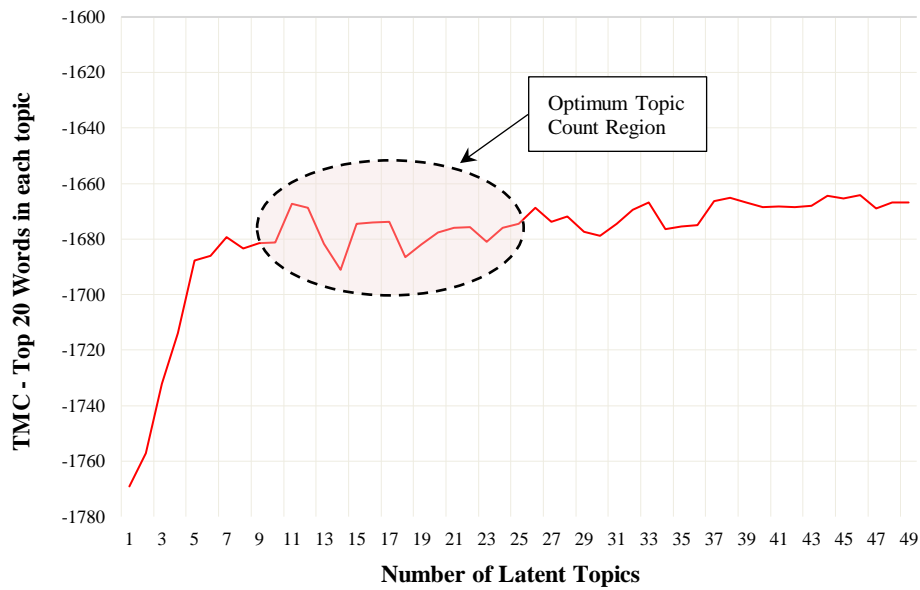
FIG. 8: GMM Topic Coherence Testing
