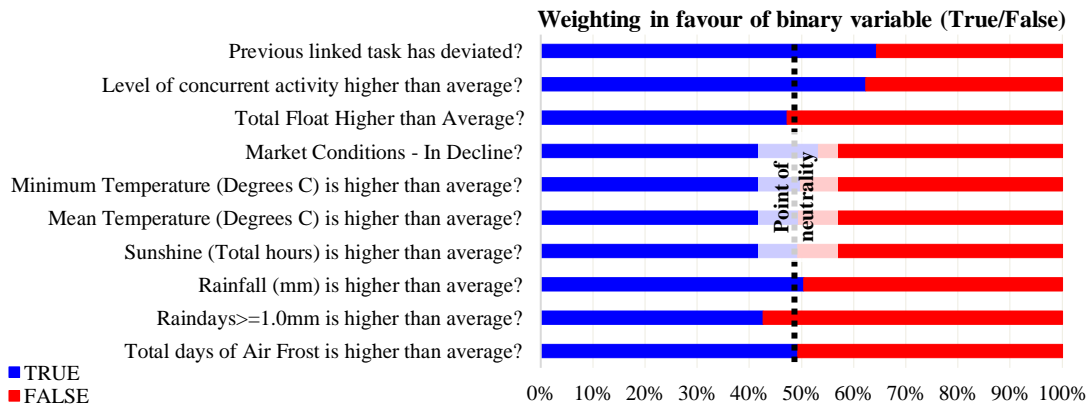
FIG. 11: Task Duration Deviation Probability by Measured Feature
