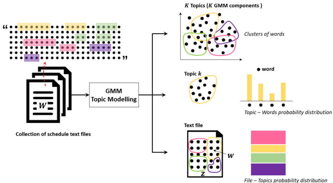
FIG. 3: The tasks of GMM Topic Modelling
