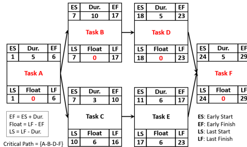
FIG. 4: The CPM-DAG network
