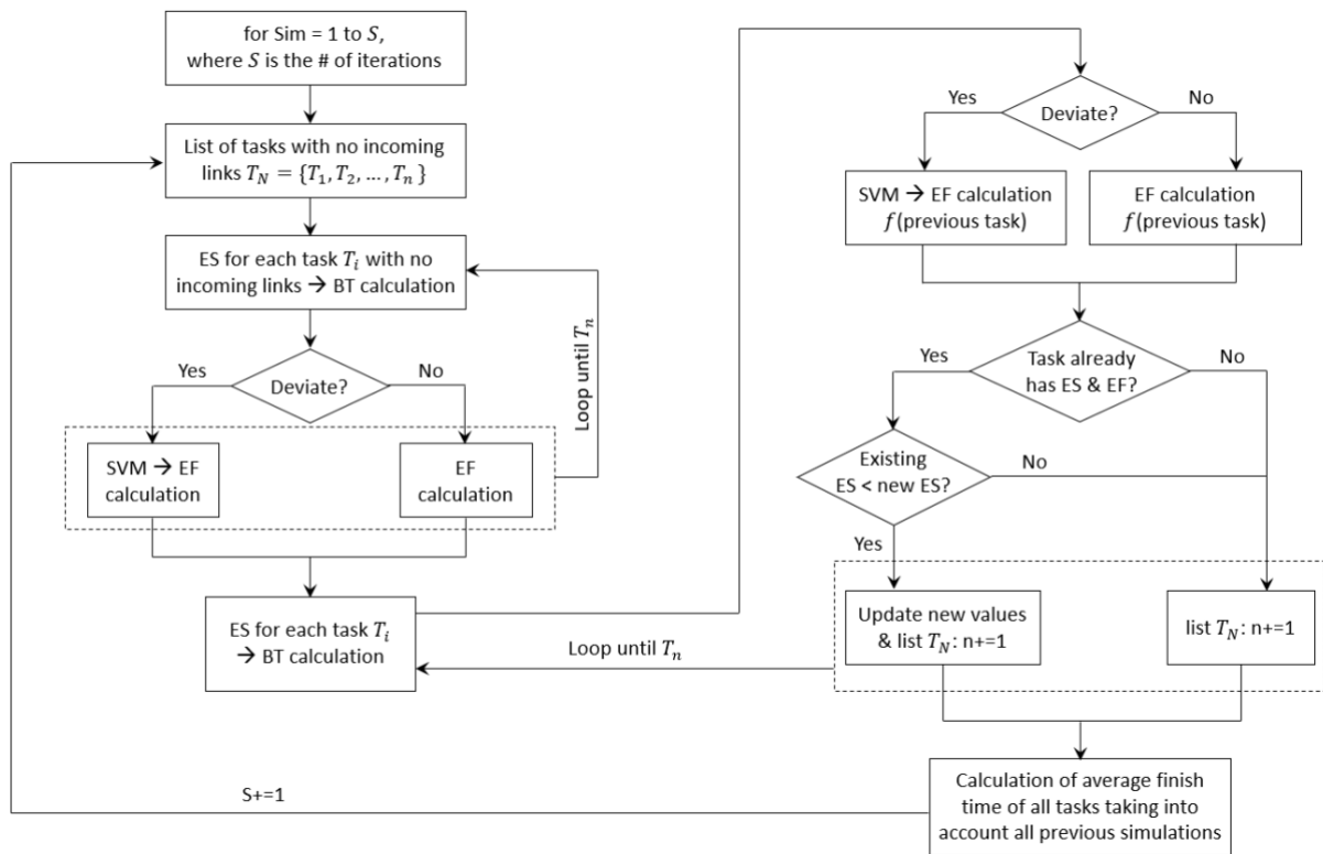
FIG. 6: Proposed Risk Simulation
