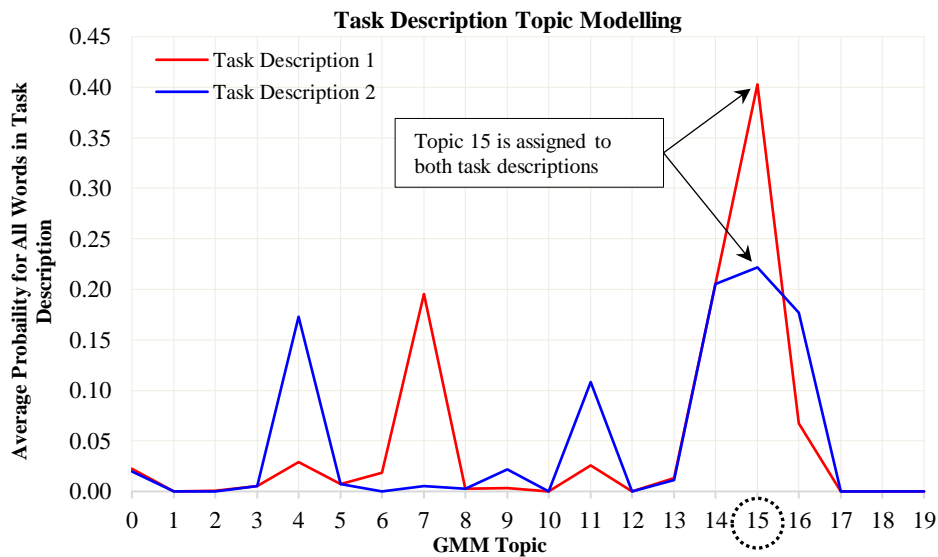
FIG. 9: Topic probability distributions for 2 task descriptions
