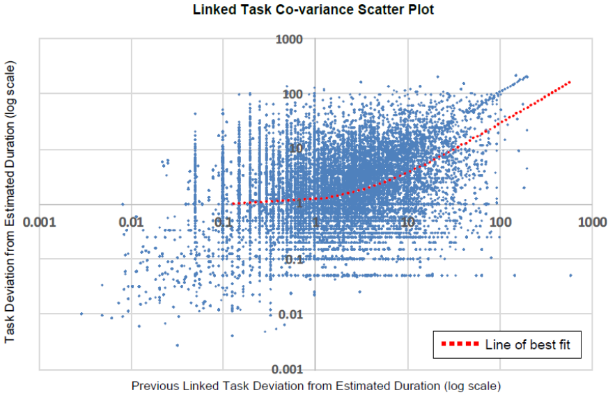
FIG. 13: Covariance between linked tasks
