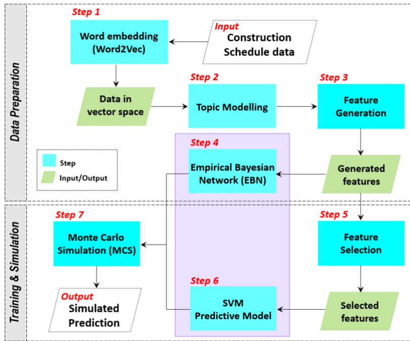
FIG. 1: Workflow of the proposed machine learning method
