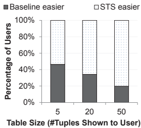
Fig. 14: Summary - Readability
