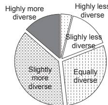
Fig. 12: Selection - Diversity
