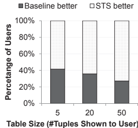
Fig. 15: Summary - Preference
