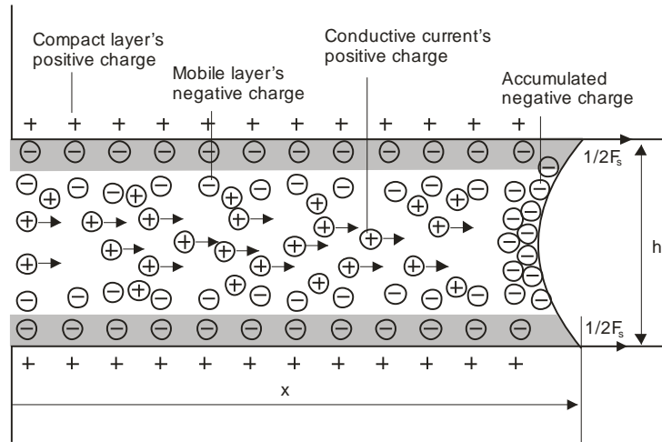
Figure 1. Capillary filling in a nanochannel: Ions distribution and movement inside a liquid column moving in a nanochannel due to capillary filling
