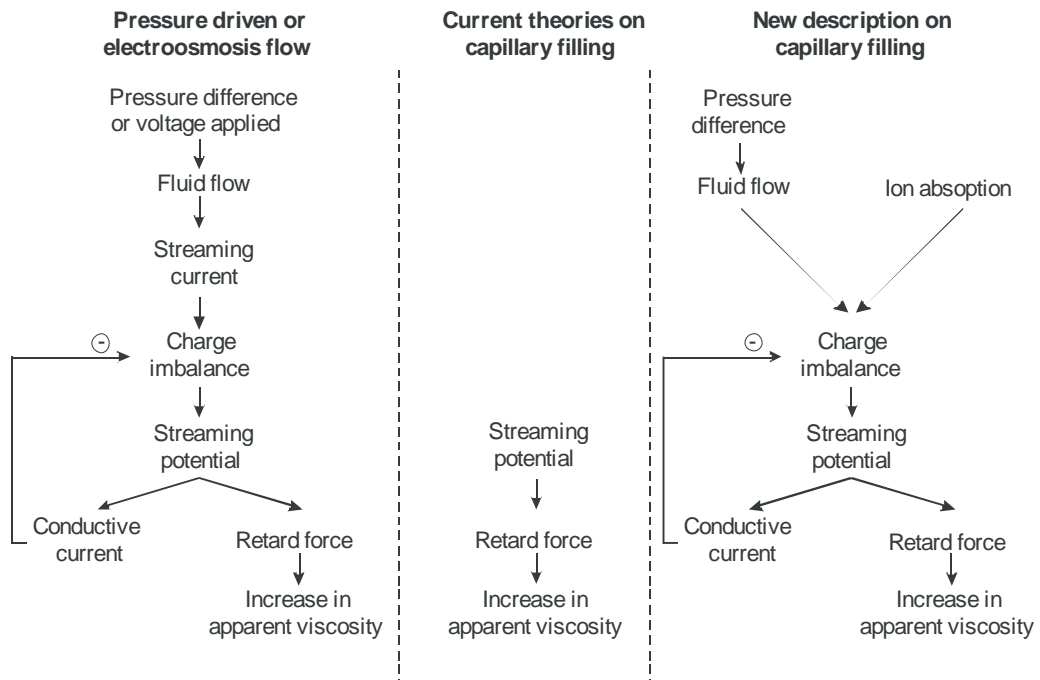
Figure 2: Comparison of existing theoretical approaches for analyzing the increase of apparent viscosity and the present analysis on capillary filling
