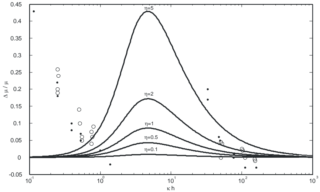
Figure 6 Ratio \Delta\mu/\mu versus normalized channel height with different \eta . The white circles show experimental results from (Tas et al., 2004). The black dots show experimental results from (Persson et al., 2007)
