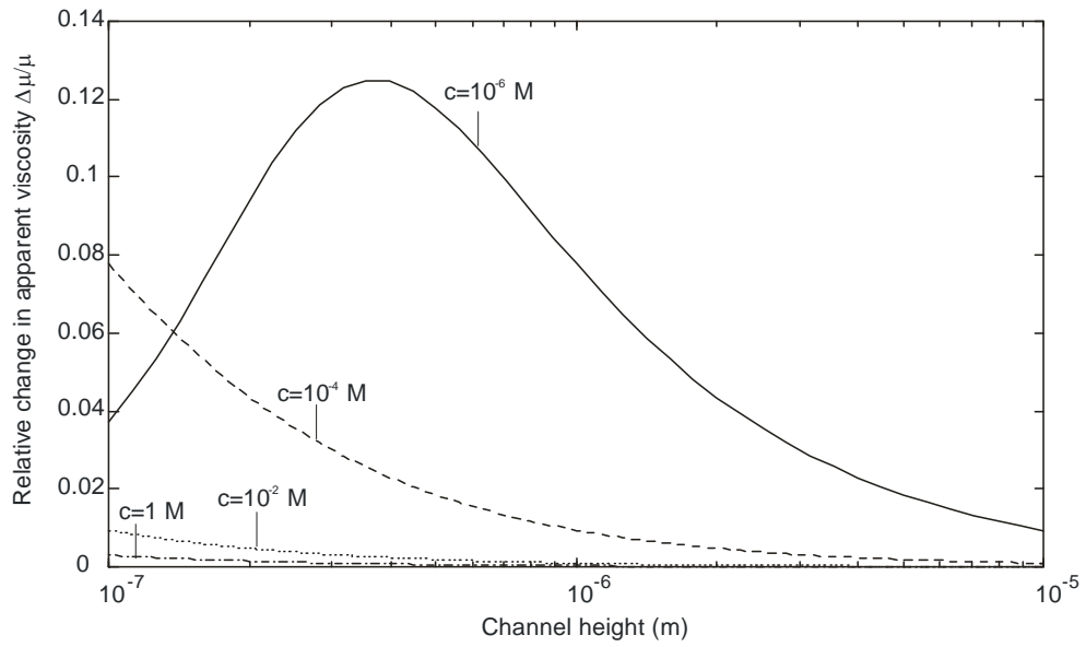
Figure 5 Ratio \Delta\mu/\mu versus channel height at different concentrations.
