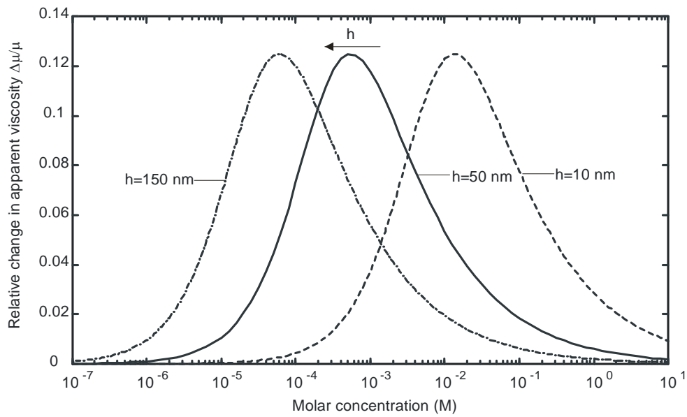
Figure 4 Ratio \Delta\mu/\mu versus concentration at different channel heights.
