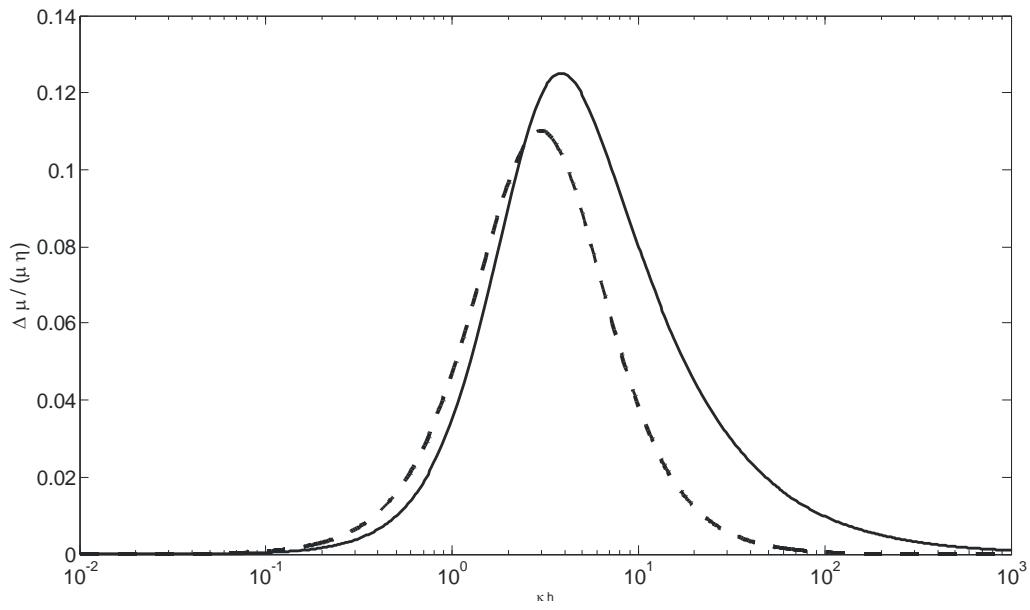
Figure 7 Ratio \Delta\mu/(\mu\eta) versus normalized channel height. The solid line shows results derived from equation (37). The dashed line shows corresponding results from (Mortensen and Kristensen, 2008)
