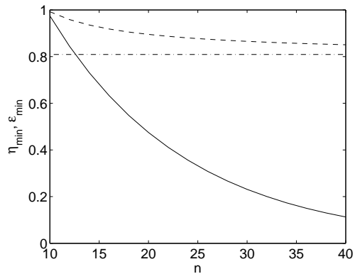
Figure 1: Minimum state preparation fidelity \epsilon_{min} for ideal detectors (solid line), and minimum detection efficiency \eta_{min} for ideal state preparation (dashed line) required for violation of (8) as a function of the number of modes. The asymptotic value of \eta_{min} is indicated by the dash-dotted line.
