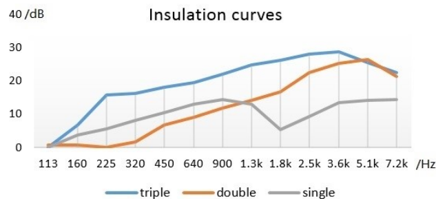
Figure 3 – Frequency attenuation (insulation curve after calculation).
