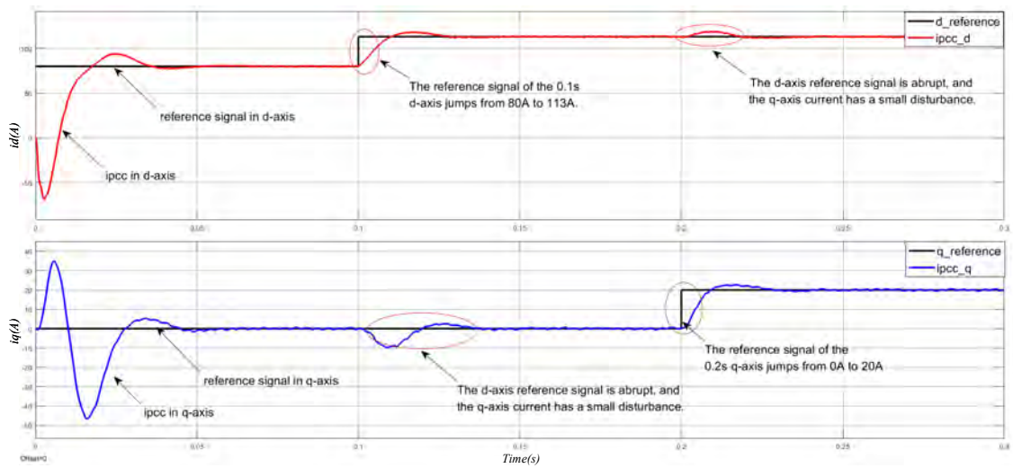
Figure 12. The point of common coupling current response curve of Scheme I.
