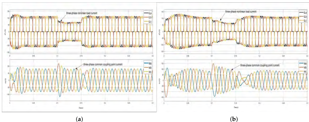
Figure 14. (a) Three-phase nonlinear load current and grid current of Scheme I; (b) three-phase nonlinear load current and grid current of Scheme II.
