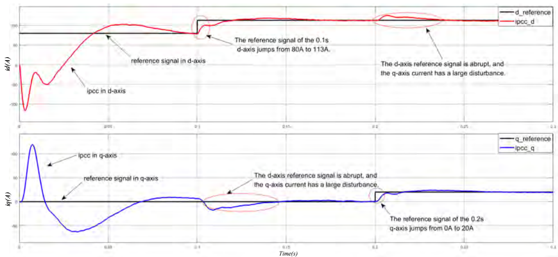
Figure 13. The point of common coupling current response curve of Scheme II.
