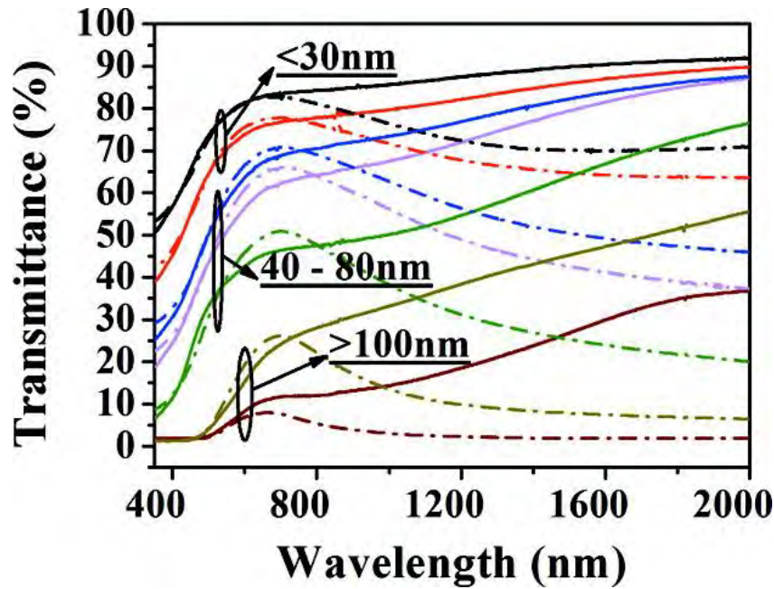
Figure 3. UV-Vis-NIR transmittance spectra for VO 2 continuous films with different thickness. The solid and dashed lines represent the spectra measured at 20 and 90 °C, respectively. It is apparent that an ultrathin VO 2 film (<30 nm) can provide high T_{lum} (~80%) but low \Delta T_{solar} (~20%). With the increased film thickness (> 100 nm), \Delta T_{solar} was noticeably enhanced (~50%) while T_{lum} was dropped sharply (~10%). Reproduction from [27] with permission from American Chemical Society, Copyright 2010.
