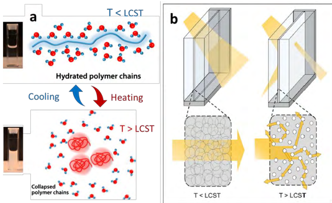
Figure 6. Schematic of thermochromic hydrogels below and above the LCST. (a) The temperature-responsive arrangement of polymer chains. Below the LCST, the hydrophilic polymer chains are surrounded by water molecules and the hydrogel is transparent. Above the LCST, the polymer chains lose water molecules and collapse into polymer clusters which makes the hydrogel opaque. Reproduction from [65] with permission from Elsevier, Copyright 2016. (b) The schematic of a smart window where the thermochromic hydrogel layer is sandwiched between two glass panels. The incident light can pass through the hydrogel layer below the LCST but is largely blocked above the LCST due to the light scattering. Reproduction from [42] with permission from Elsevier, Copyright 2019.
