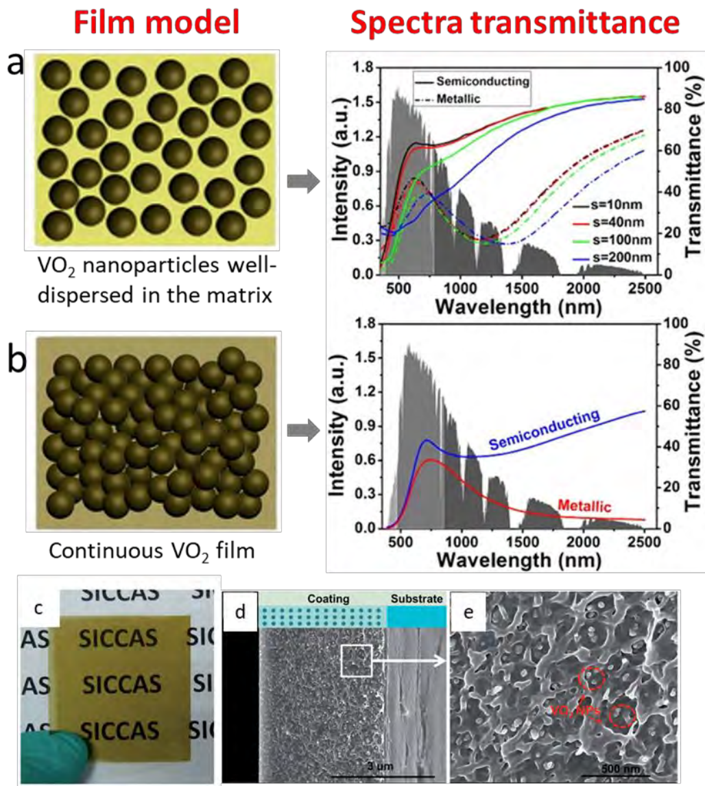
Figure 4. The simulated and the experimental dispersive \text{VO}_2 nanocomposites. The ideal film models and their simulated light transmittance spectra for (a) a nanocomposite in which \text{VO}_2 nanoparticles (with different sizes: 10, 40, 100 and 200 nm, filling factor = 0.01) are uniformly embedded and (b) the continuous film in which the \text{VO}_2 nanoparticles cluster together. With the same film thickness of 10 \mu\text{m} , the dispersive \text{VO}_2 nanocomposite obviously has advantages in high \Delta T_{\text{solar}} and T_{\text{lum}} over the continuous film. (a-b) Reproduction from [40] with permission from American Chemical Society, Copyright 2015. (c) The image of the nanocomposite coated glass which shows yellowish green colour. The composite coating is composed of the dispersed \text{VO}_2 nanoparticles in the PU matrix. (d) SEM images of the cross-sectional nanocomposite coating on the substrate and (e) the homogeneous dispersion of \text{VO}_2 nanoparticles in the PU matrix. (c-e) Reproduction from [30] with permission from Royal Society of Chemistry, Copyright 2014.
