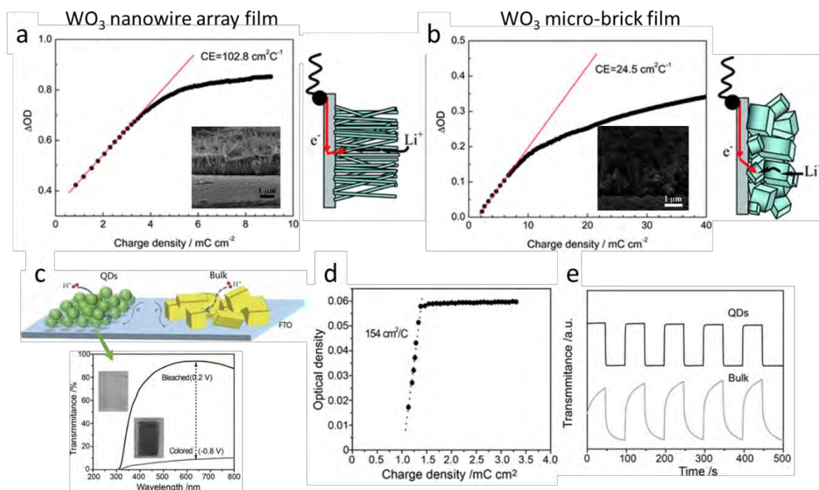
Figure 12. Nanocrystalline WO 3 in the form of nanowires and quantum dots and the corresponding electrochromic performance. Colouration efficiency of WO 3 nanowire array film (a) and WO 3 micro-brick film (b). Reproduction from [108] with permission from Royal Society of Chemistry, Copyright 2011. (c) Tungsten oxide QDs provide more efficient ion diffusion and charge transfer than the bulk counterpart. Transmittance spectra for tungsten oxide QDs electrode deposited on FTO glass in the coloured (-0.8 V) and bleached (+0.2 V) states, respectively. The electrochromic window is highly transparent at bleached state (> 90% of transmittance) and large modulation window (> 80%). The insets are images of the electrode at bleached and coloured states, appearing almost transparent and dark blue colour, respectively. (d) The colouration efficiency of the QDs-based electrochromic window. (e) Alternate transmittance switching for bulk (green) and QDs (black) tungsten oxide showing the significant faster response for QDs. Reproduction from [103] with permission from Wiley-VCH, Copyright 2014.
