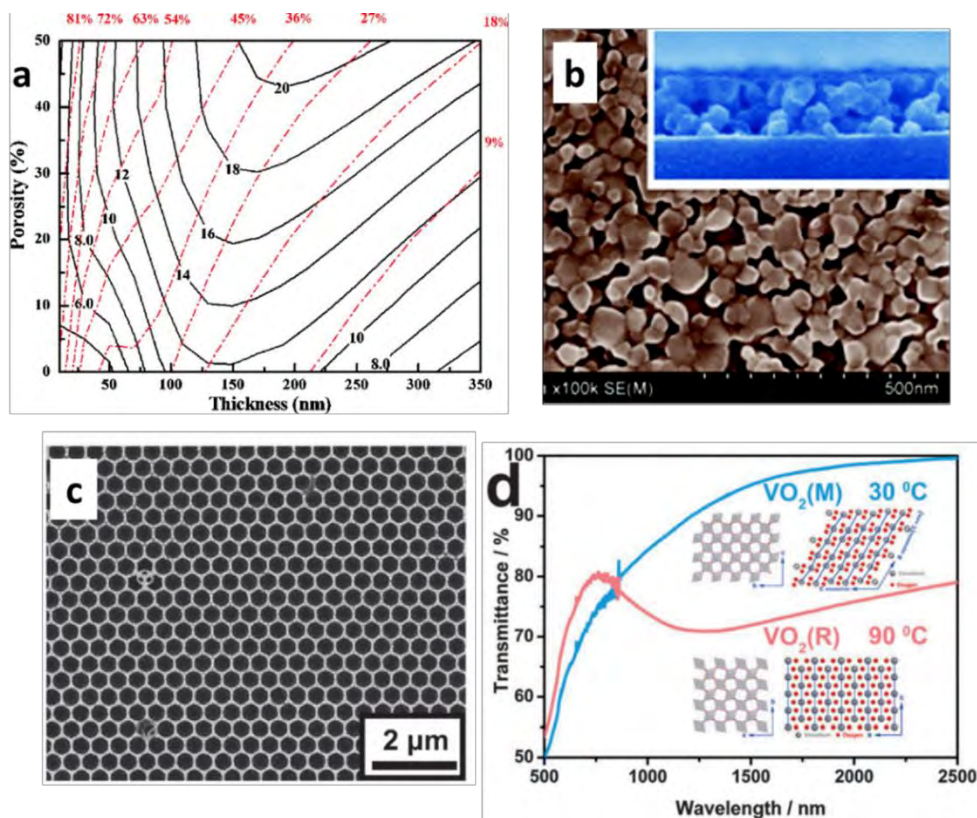
Figure 5. The simulated and experimental optical performance of nanoporous VO 2 film. (a) The calculated T_{lum} of monoclinic VO 2 at low temperature (red dotted lines) and \Delta T_{solar} of rutile VO 2 at high temperature (black solid lines) as a function of thickness and porosity of the VO 2 films. (b) SEM image of the VO 2 film with random porosity. The inset is the cross-sectional view of the nanoporous film. (a-b) Reproduction from [25] with permission from American Chemical Society, Copyright 2011. (c) SEM image of the single layered periodic porous VO 2 film (3) The spectral transmittance of the periodic porous film at low temperature insulating (M phase, 30 °C) and high temperature metallic state (R phase, 90 °C). It is apparent that the porous VO 2 highlights the ultrahigh visible transmittance regardless of the phase transition ( T_{lum} > 80%). (c-d) Reproduction from [45] with permission from Royal Society of Chemistry, Copyright 2014.
