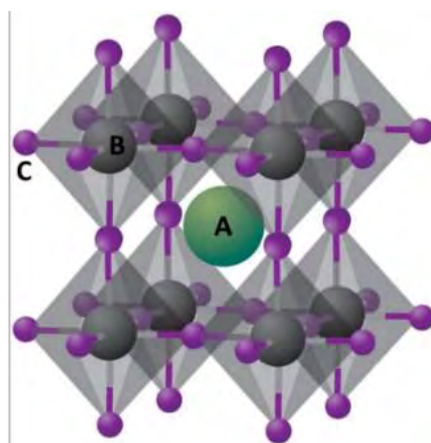
Figure 9. Crystal structure of cubic halide perovskites with the general formula of ABX_3 . The larger cation A (green) occupied the cuboctahedral voids formed by the 12 nearest-neighbouring X ions (purple). The smaller cation B is centred at the unit cell. Reproduction from [70] with permission from Nature Publishing Group, Copyright 2014.
