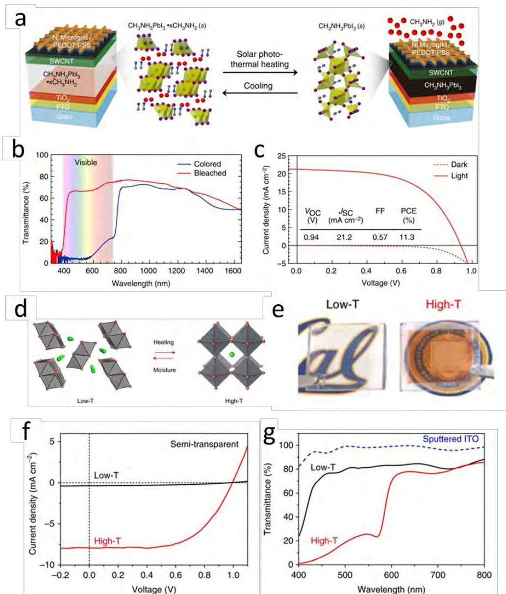
Figure 11. The halide perovskite smart solar windows based on the complexation-dissociation of methylamine (a-c) and the temperature-responsive structural change (d-g). (a) Schematic of the smart solar window architecture and the chemical-reaction induced thermochromism. In the architecture, \text{TiO}_2 is the electron transport layer and fluorine-doped tin oxide (FTO) is the transparent conducting electrode. The single-walled carbon nanotube (SWCNT) is to provide hole extraction and improve lateral electrical transport. The topmost layer (microgrid/PEDOT:PSS) serves as an electric glue to package the whole device. (b) Transmittance spectra of the smart solar window in the transparent (red) and opaque (blue) states. It is obvious that the visible transmittance sharply drops after the dissociation of methylamine from the perovskite. (c) Current density vs voltage curve of the switchable smart solar window in the dark (dashed) and under illumination (solid). Reproduction from [75] with permission from Nature Publishing Group, Copyright 2017. (d) Schematic of the thermally driven, moisture-mediated reversible phase transition between the high-T and low-T phases. (e) The picture of the \text{CsPbI}_3 smart solar window in the colourless low-T state (left) and deeply coloured high-T state (right). The sputtered indium tin oxide (ITO) layer acts as the top transparent electrodes. (f) Current density vs voltage curve of the device. (g) The transmittance spectra of the smart solar windows at low-T (black) and high-T state (red). The spectrum for the sputtered ITO layer is as a reference. Reproduction from [78] with permission from Nature Publishing Group, Copyright 2018.
