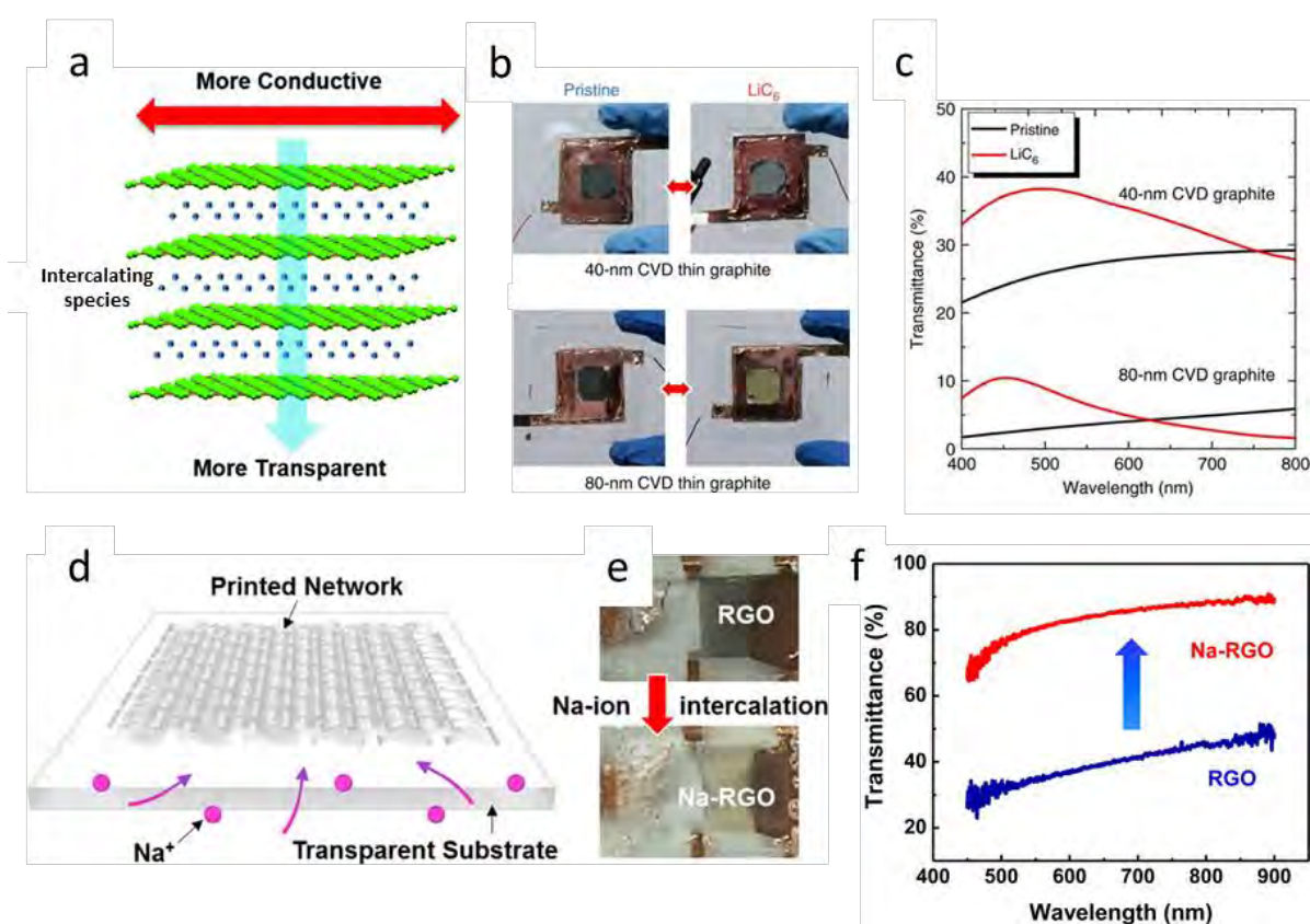
Figure 14. The intercalated graphene based electrochromic device. (a) Schematic of the multilayered graphene intercalated by metal ions. Reproduction from [132] with permission from Royal Society of Chemistry, Copyright 2016. (b) Images of the encapsulated CVD graphene electrochromic device with different thickness of graphene electrode. (c) The optical transmittance before and after the \text{Li}^+ intercalation. Both CVD graphene electrodes showed the increased transparency after applying the external voltage to the devices. Reproduction from [137] with permission from Nature Publishing Group, Copyright 2014. (d) Schematic of \text{Na}^+ intercalation in the rGO film on the transparent substrate. (e) The images show the transparency increase in the \text{Na}^+ -intercalated rGO electrochromic device. (f) The optical transmittance of rGO film before and after \text{Na}^+ intercalation. Reproduction from [139] with permission from American Chemical Society, Copyright 2015.
