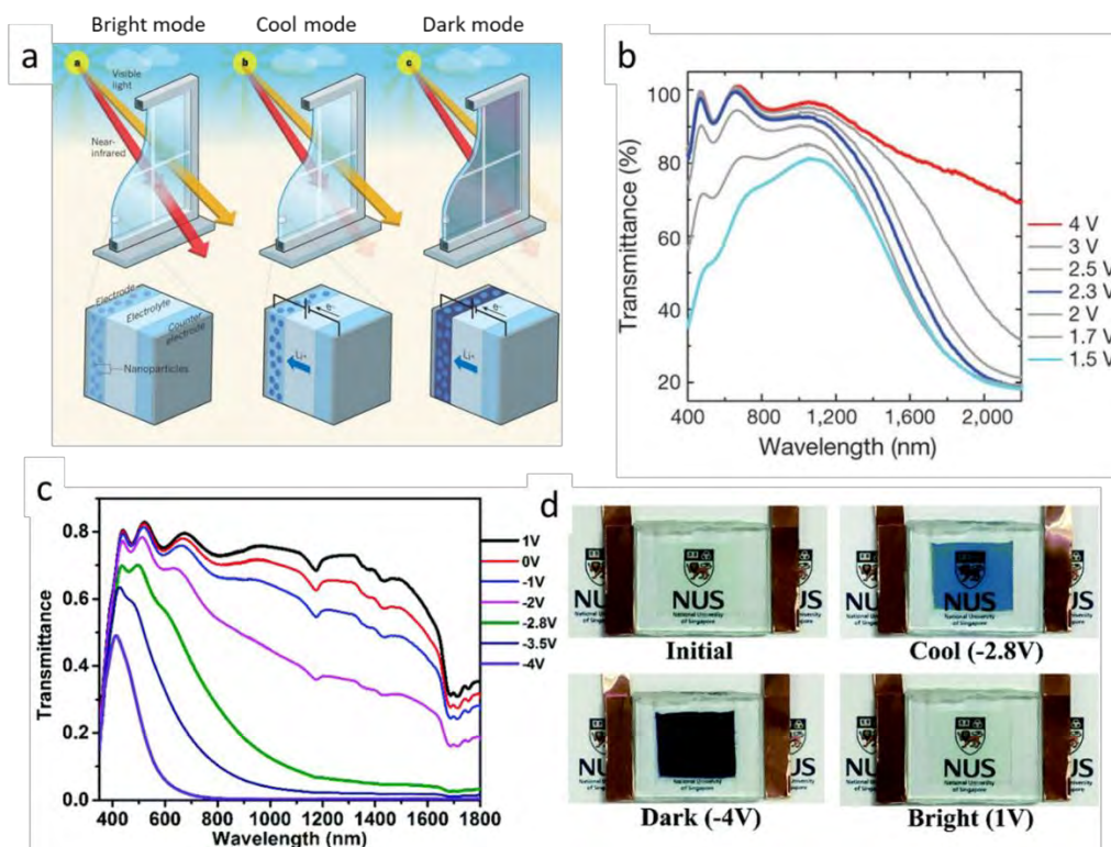
Figure 13. The dual-band smart windows which can dynamically and independently manage the transmission of visible and NIR light. (a) The smart window based on plasmonic nanocrystal-in-glass exhibits three distinct modes. Reproduction from [125] with permission from Nature Publishing Group, Copyright 2013. (b) Changes in the transmittance spectra of the ITO-in-NbO x film with the varying voltages versus Li/Li + . The composite shows bright mode at 4 V, cool mode at 2.3 V and dark mode at 1.5 V. Reproduction from [114] with permission from Nature Publishing Group, Copyright 2013. (c) The transmittance spectra of the m-WO 3-x nanowires-based dual-band smart window under different external biases. (d) The three modes under different voltage. Reproduction from [123] with permission from Royal Society of Chemistry, Copyright 2018.
