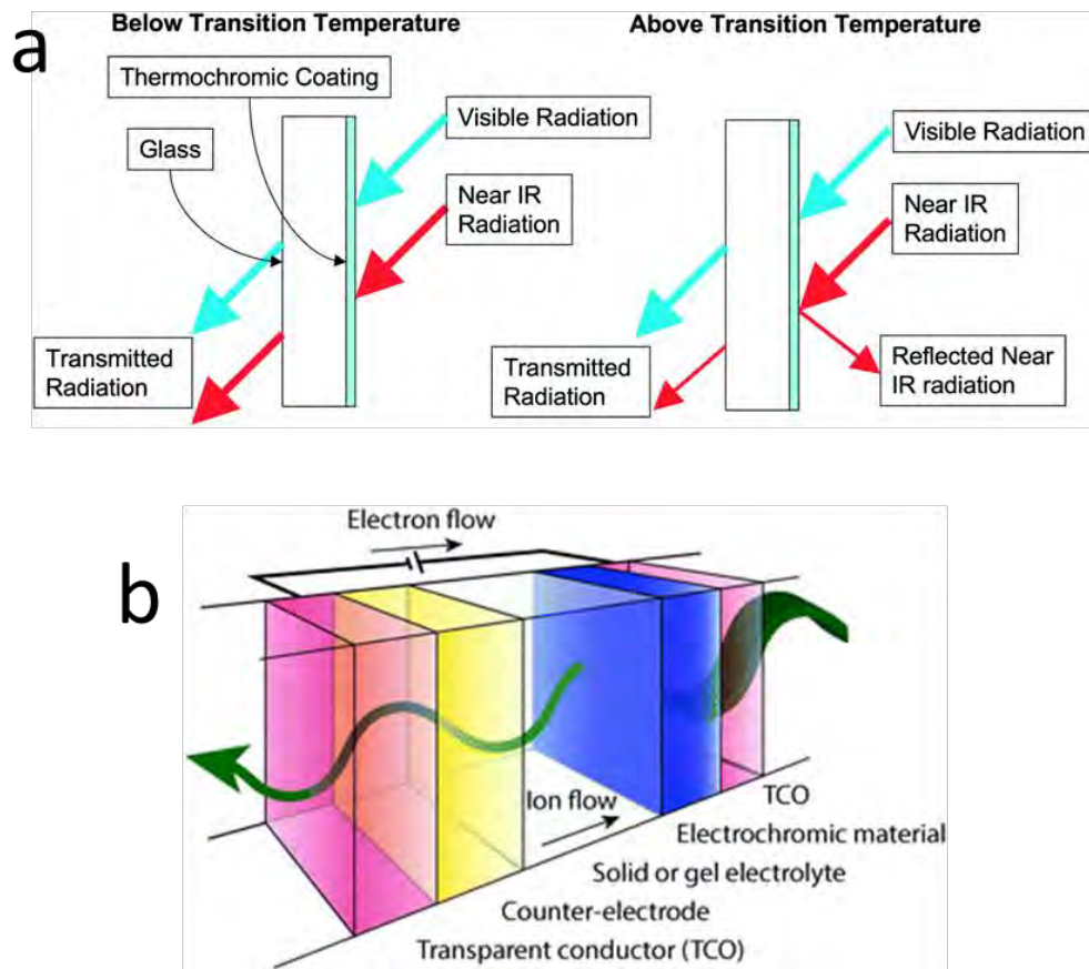
Figure 1. The schematic mechanism of thermochromic and electrochromic windows. (a) For the thermochromic windows, the active thermochromic coating has a critical transition temperature. Below the transition temperature, most of the NIR light can pass through the window, thus transferring the solar heat into the building (keep the interior warm). However, the NIR light will be blocked outdoors above the transition temperature, which greatly reduces the transmitted heat radiation (keep the interior cool). Reproduction from [4] with permission from Royal Society of Chemistry, Copyright 2014. (b) When applying the voltage, the flowing ions will cause the reversible chromogenic reaction in the electrochromic layers, contributing the colour changes. Reproduction from [2] with permission from Royal Society of Chemistry, Copyright 2014.
