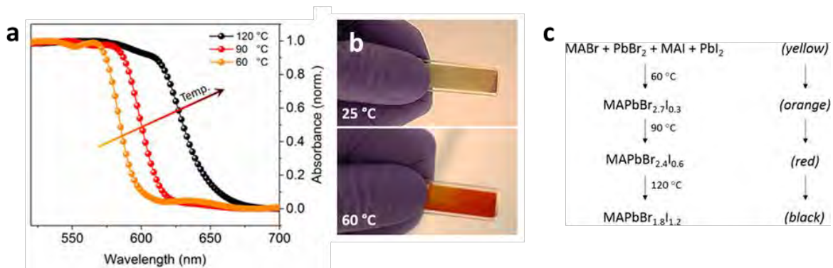
Figure 10. (a) Absorption spectra of thermochromic perovskite crystals obtained at 60, 90 and 120 °C. The original yellow solution changed to orange at 60 °C, to bright red at 90 °C, and finally to black at 120 °C. (b) Images of the thermochromic prototype annealed at 25 and 60 °C. (c) The formulation of the original perovskite solution and the major contributors of colour changes at 60, 90 and 120 °C. Reproduction from [71] with permission from American Chemical Society, Copyright 2017.
