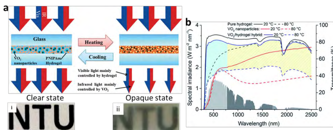
Figure 8. (a) The schematic of the smart window based on the VO 2 /PNIPAm nanocomposite. The PNIPAm matrix regulates the visible transmittance at ~30 °C while VO 2 nanoparticles regulate the NIR transmittance at ~68 °C. The insets (i) and (ii) show the clear state at room temperature (hydrated PNIPAm) and opaque state at 35 °C (dehydrated PNIPAm). (b) UV-Vis-NIR transmittance spectra of VO 2 /PNIPAm nanocomposite, pure VO 2 nanoparticles and pure PNIPAm at 20 and 80 °C. It is obvious that VO 2 /PNIPAm hybrid has higher T_{lum} than pure VO 2 due to the reduced light scattering. Further, VO 2 /PNIPAm hybrid has greatly enhanced \Delta T_{solar} relative to the another two. Reproduction from [64] with permission from Royal Society of Chemistry, Copyright 2015.
