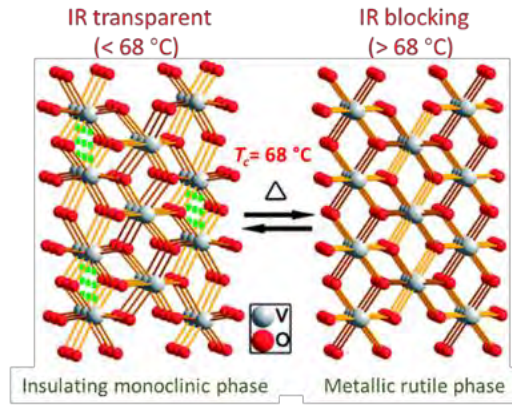
Figure 2. Schematic of the change in the crystal structure of \text{VO}_2 at the T_c of 68\text{ }^\circ\text{C} . When heated to 68\text{ }^\circ\text{C} , the insulating monoclinic \text{VO}_2 (IR transparent) will transform into the metallic rutile phase with longer V-V distance (IR blocking). Conversely, the rutile \text{VO}_2 can recover to the monoclinic phase as cooled to below T_c . Reproduction from [11] with permission from Royal Society of Chemistry, Copyright 2011.
