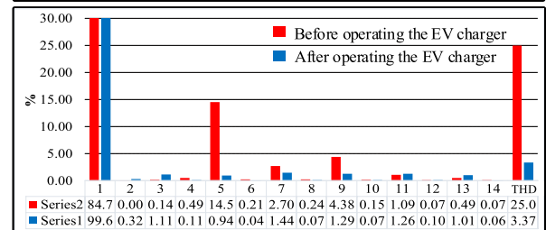
FIGURE 21. A) STATCOM and APF operation [Functions III and IV] when PF = 0.85 leading; EV charger supplies: P \approx 0 W, Q = 200 VAR, PF = 0.2 lagging, v_s (80 V/div), i_c (4 A/div), source current i_s (8 A/div) and load current i_L (8 A/div), b) THD of i_s before and after operating the EV charger.
